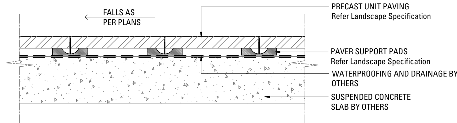
03 601 PRECAST UNIT PAVERS ON PADS ON SUSPENDED SLAB SCALE 1:10
